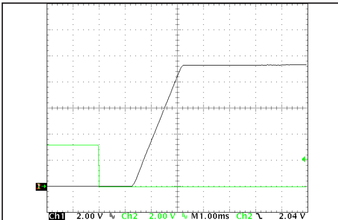
Figure 9: Turn-on transient at half load (resistive load) (1 ms/div). Load cap: 15 \mu F tantalum capacitor and 5mF ceramic capacitor bank. Input voltage pre-applied. Ch 1: V_{out} (2V/div), Ch 2: ON/OFF input (2 V/div).
