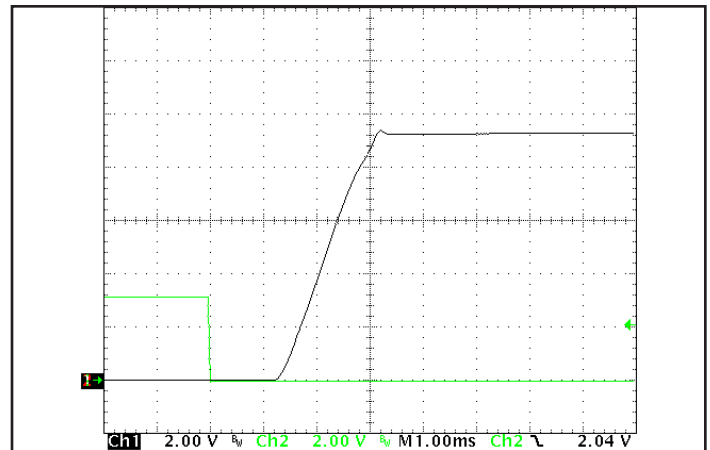
Figure 10: Turn-on transient at zero load (1 ms/div). Load cap: 15 \mu F tantalum capacitor and 5mF ceramic capacitor bank. Ch 1: V_{out} (2V/div), Ch 2: ON/OFF input (2 V/div).
