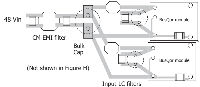
Figure H: Recommended PCB layout for input circuit
